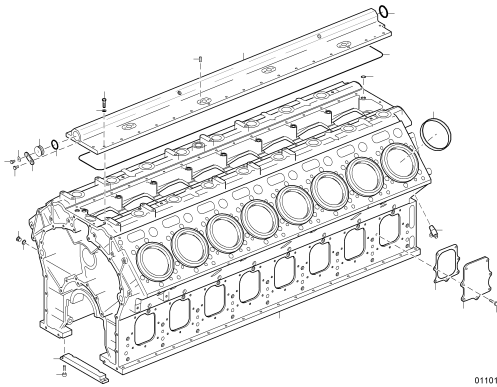
CRANKCASE UPC.06A01 2081
